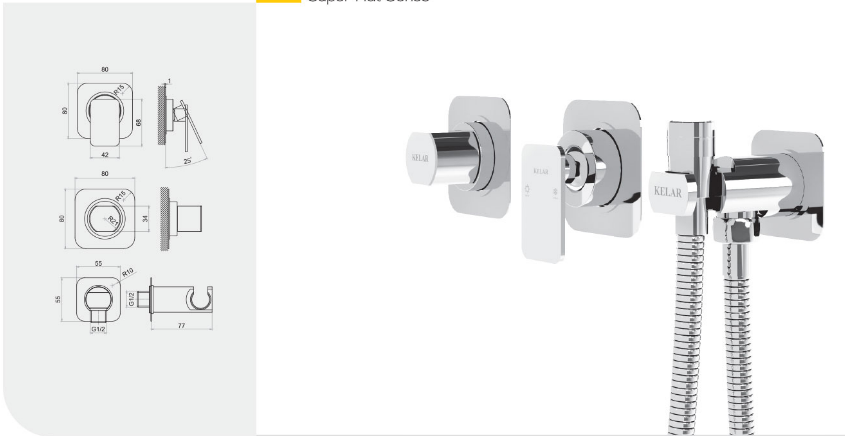
Toilet mixer Set, type Bidet Super Flat Series
