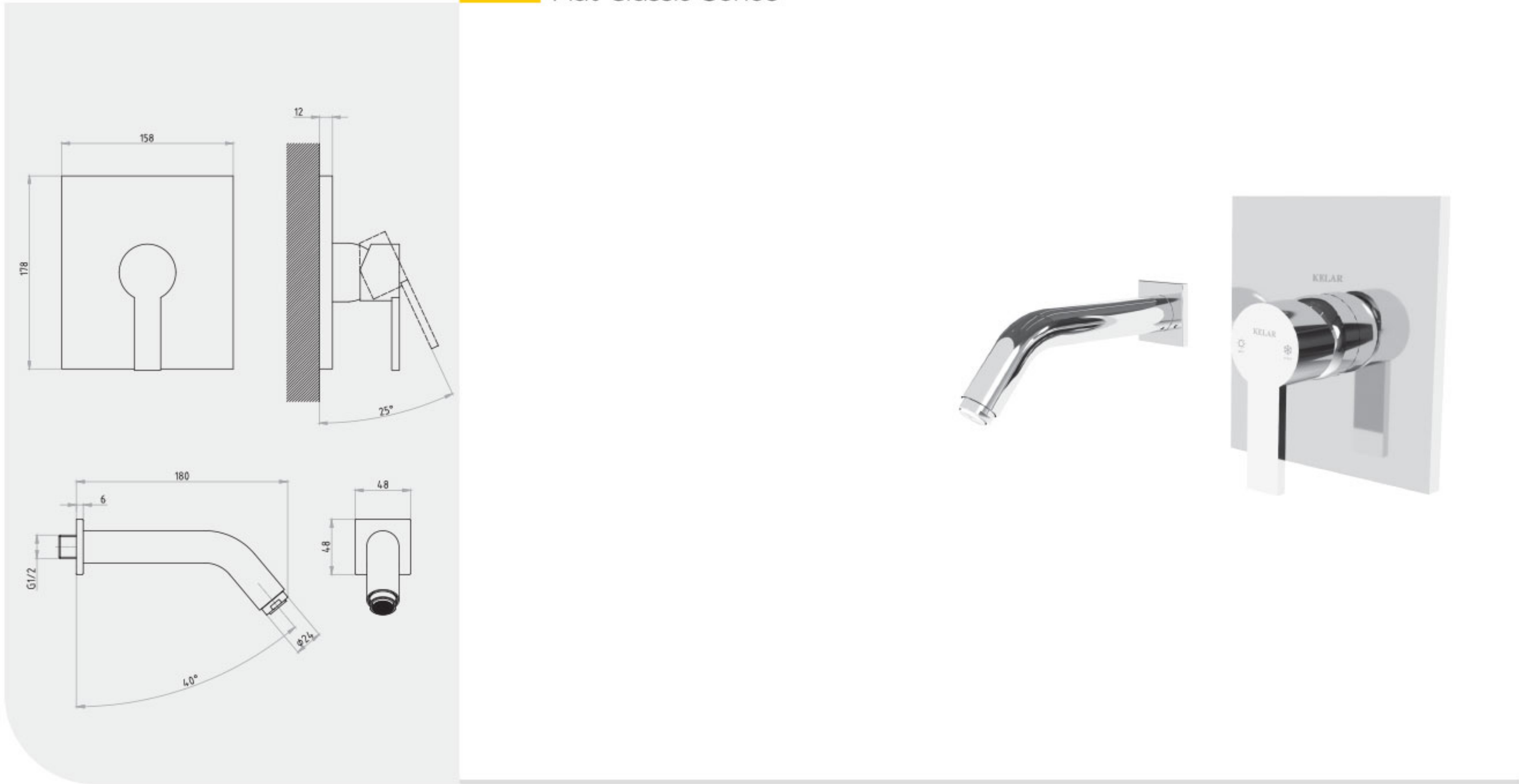
Basin mixer Set Flat Classic Series
