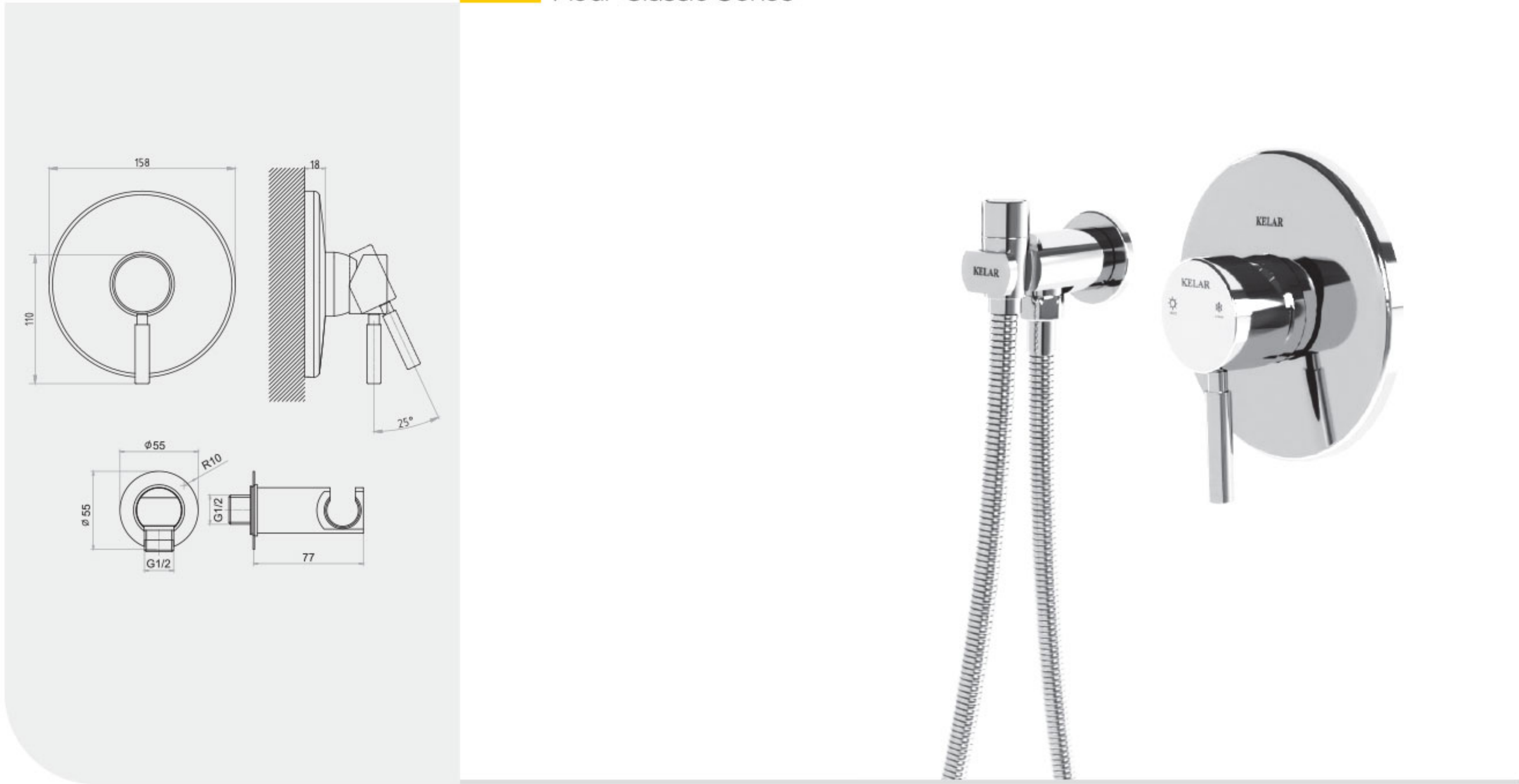
Toilet mixer Set Flour Classic Series
